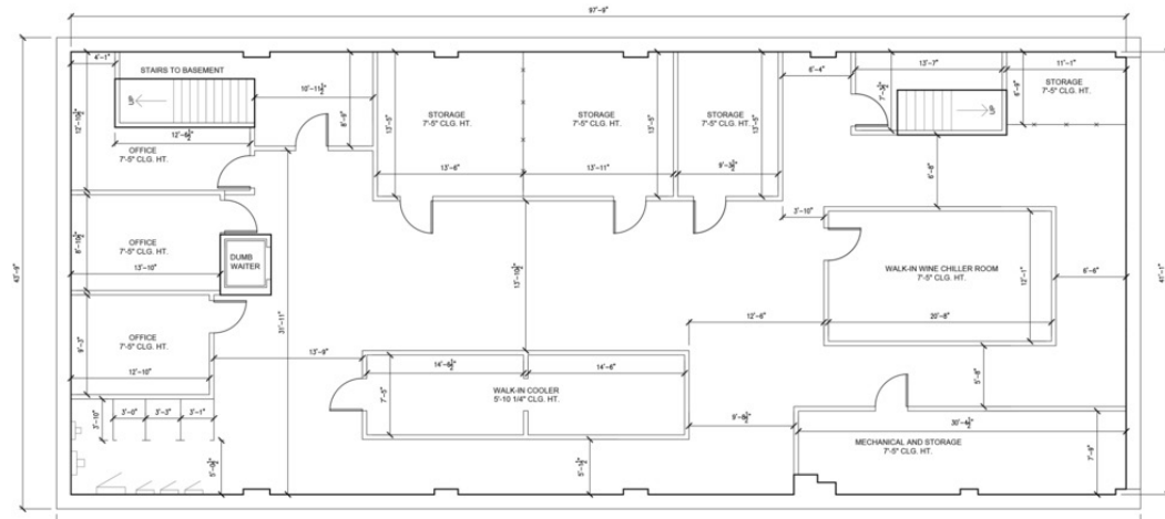
LOWER LEVEL
